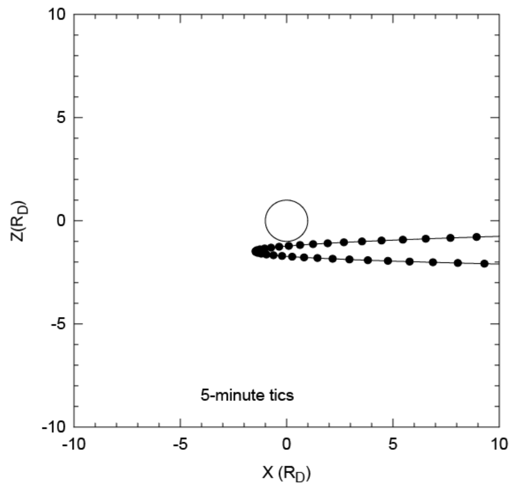
Orbit 16 Dione Flyby October 11, Day 284, 2005
