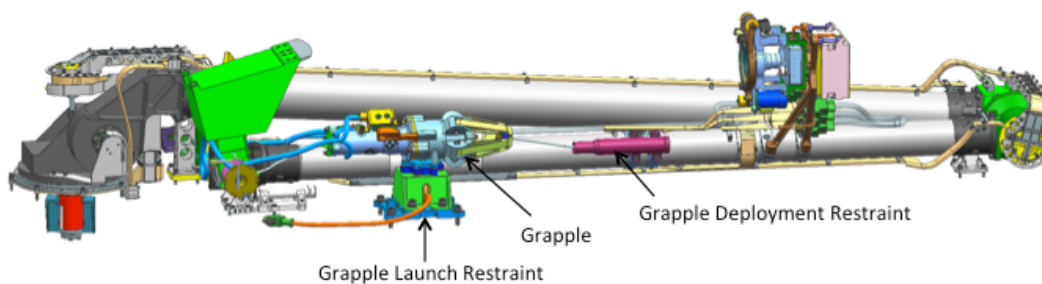
Figure 4.4.2-2: IDA and grapple stowed.
