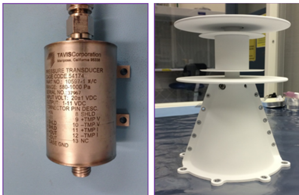
Figure 4.2.3.1-1: a) The Tavis Pressure Sensor and b) The Quad-Disc pressure sensor inlet.
