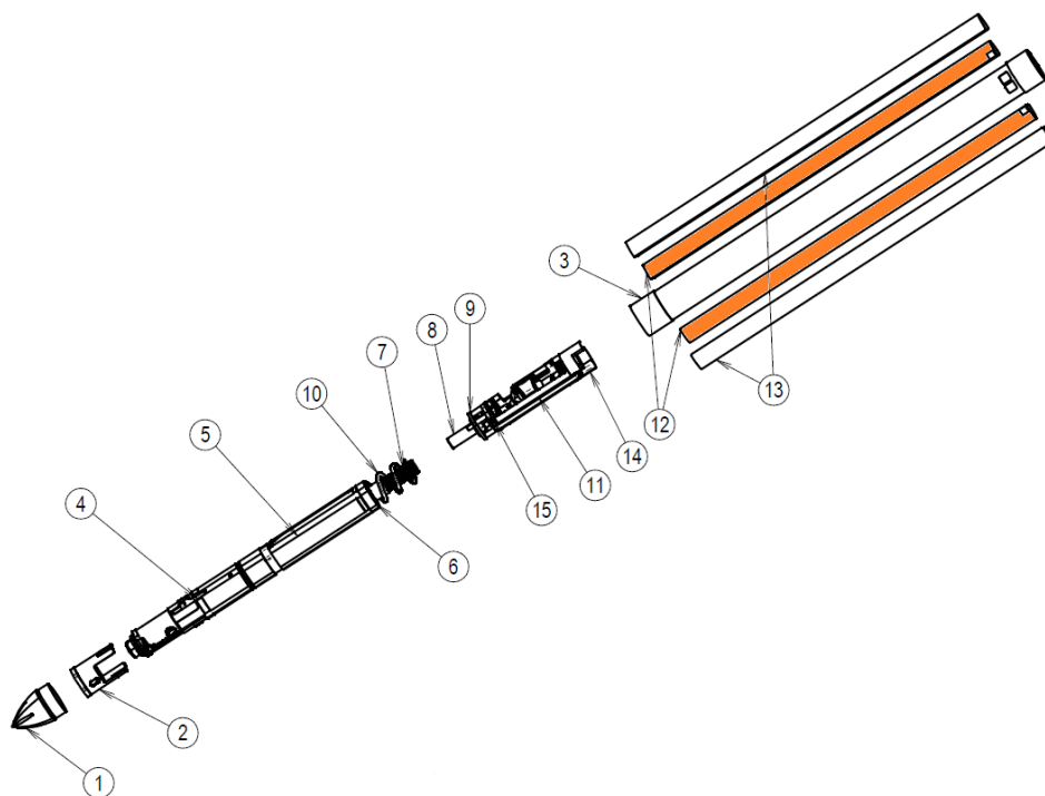
Figure 4.3.4-1: Expanded view of the mole, indicating the TEM-A heating foils (12) in orange. The foils are glued to the mole outer casing (3) and protected against abrasion by the TEM-A covers (13). Other parts refer to the hammering mechanism and STATIL assembly.
