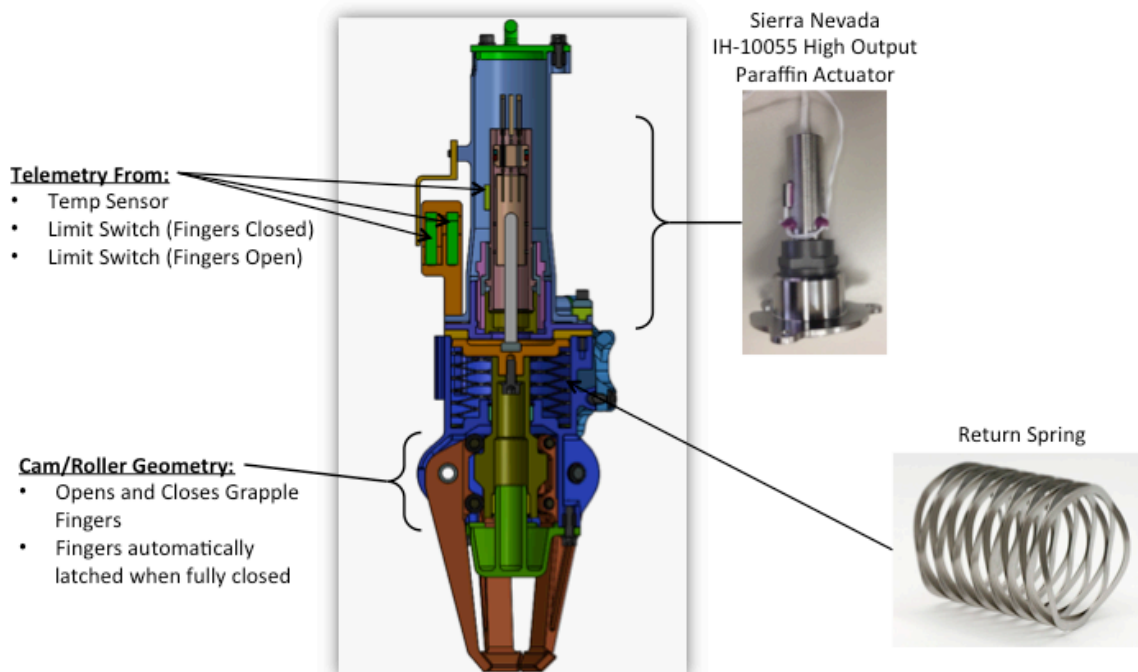
Figure 4.4.2-3: Grapple design.
